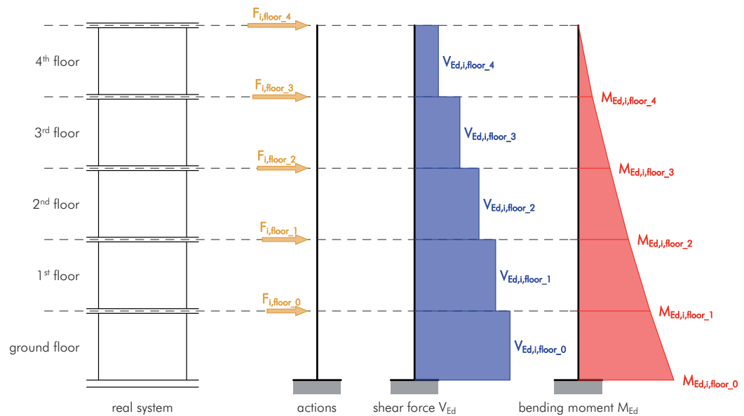
Fig. 4.2 cantilever-wall model with actions and internal forces
